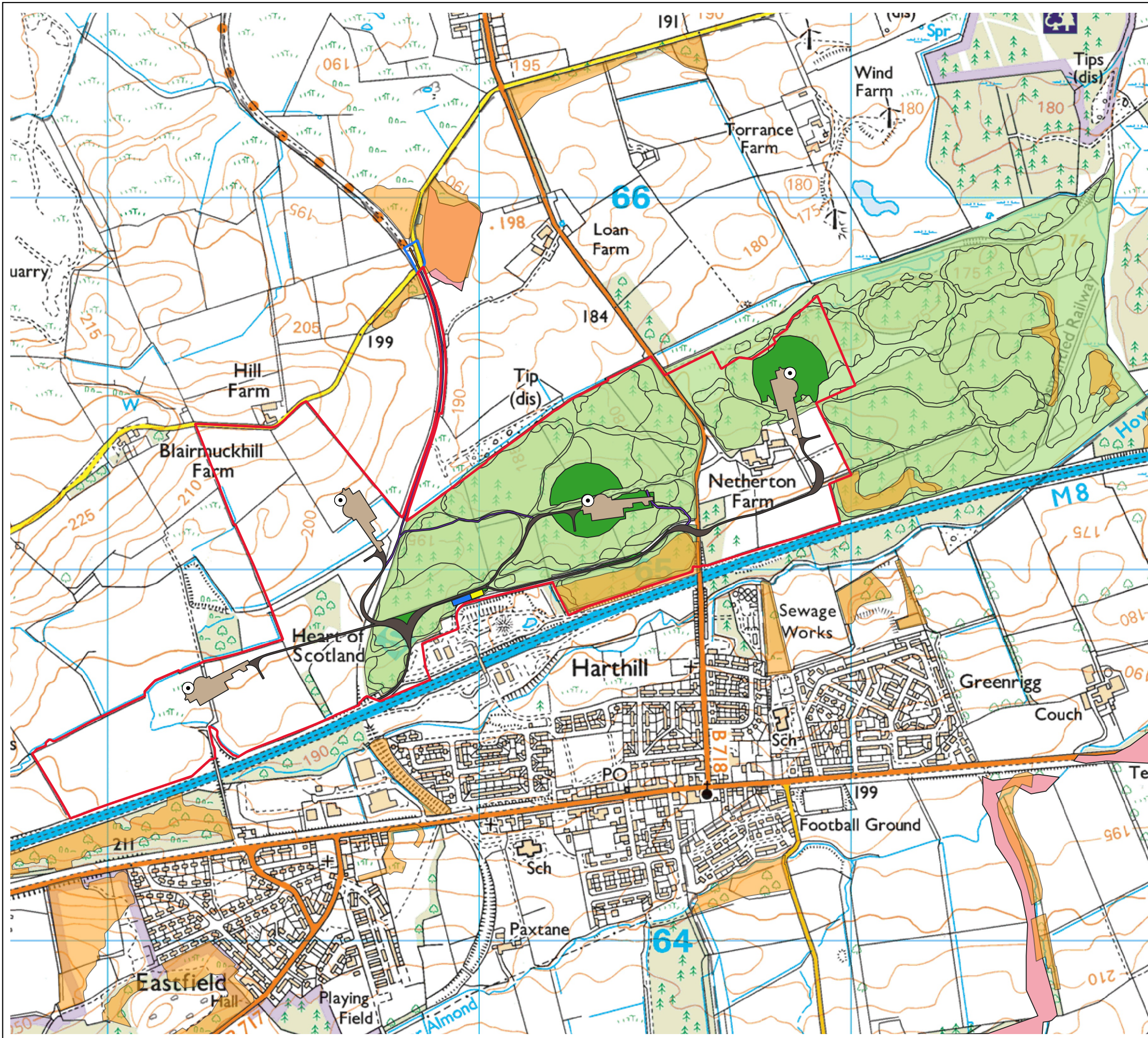
Figure No. 8.2 Wind Farm Felling Plan Torrance Wind Farm Extension II
