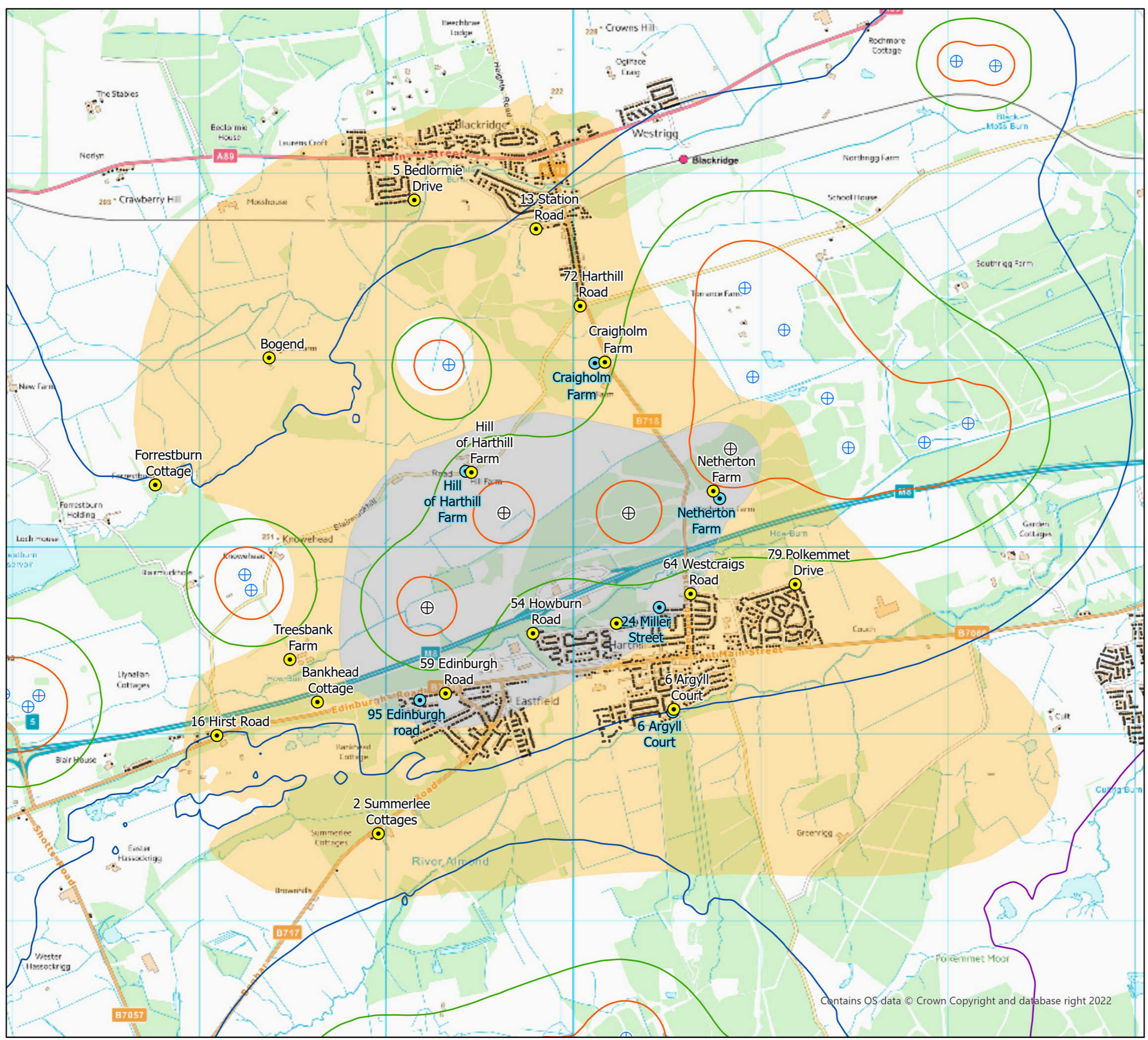
Figure 7.3 Operational Noise Assessment Torrance Wind Farm Extension II EIA Report
