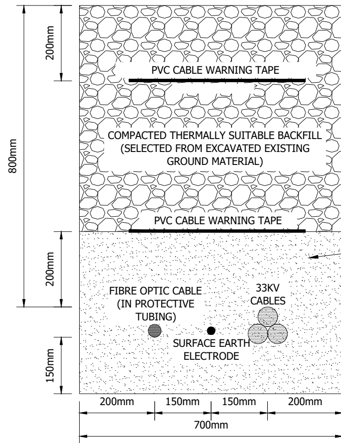
TYPICAL CABLE TRENCH DETAIL
