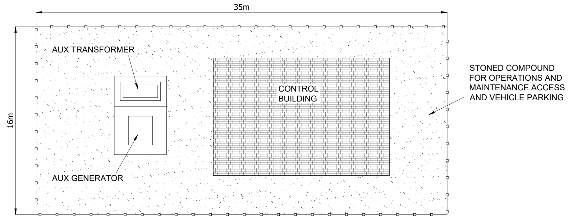
SUBSTATION COMPOUND
